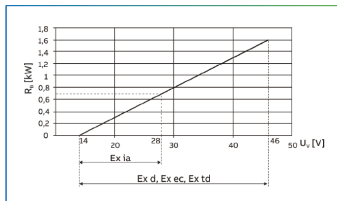
Figure 18: Terminals 31 / 32, power supply / load
