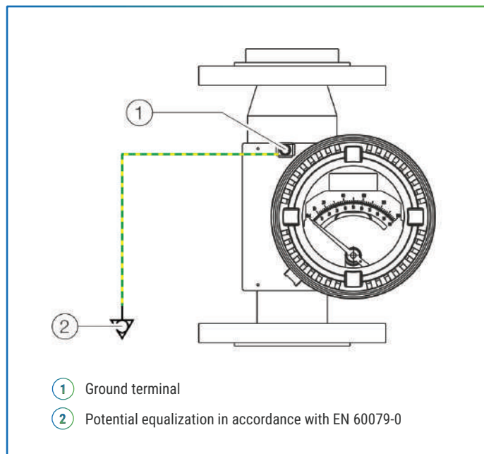
Figure 19: Grounding
