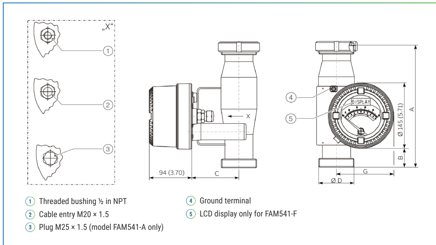
Figure 16: Dimensions in mm (in), tolerances ±2 mm
