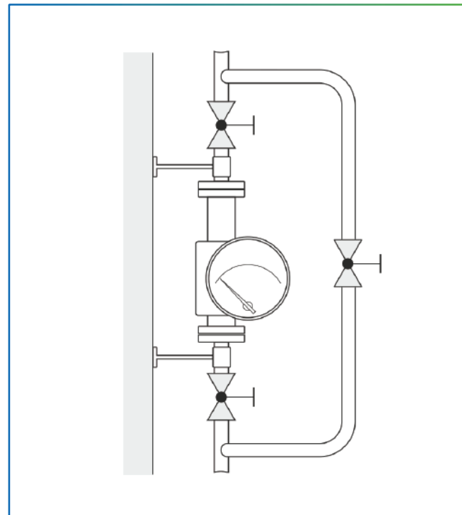
Figure 1: Installation of the flowmeter (example)
