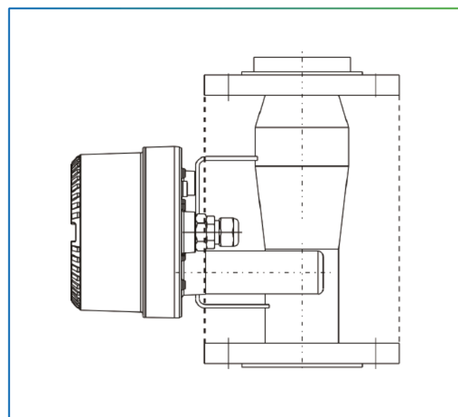
Figure 2: Insulation of the flowmeter
