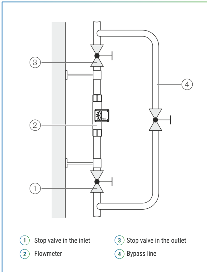
Figure 2: Installation of the flowmeter
