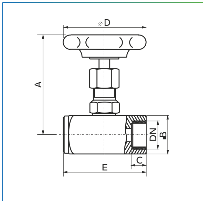
Figure 12: Stainless steel needle valve
