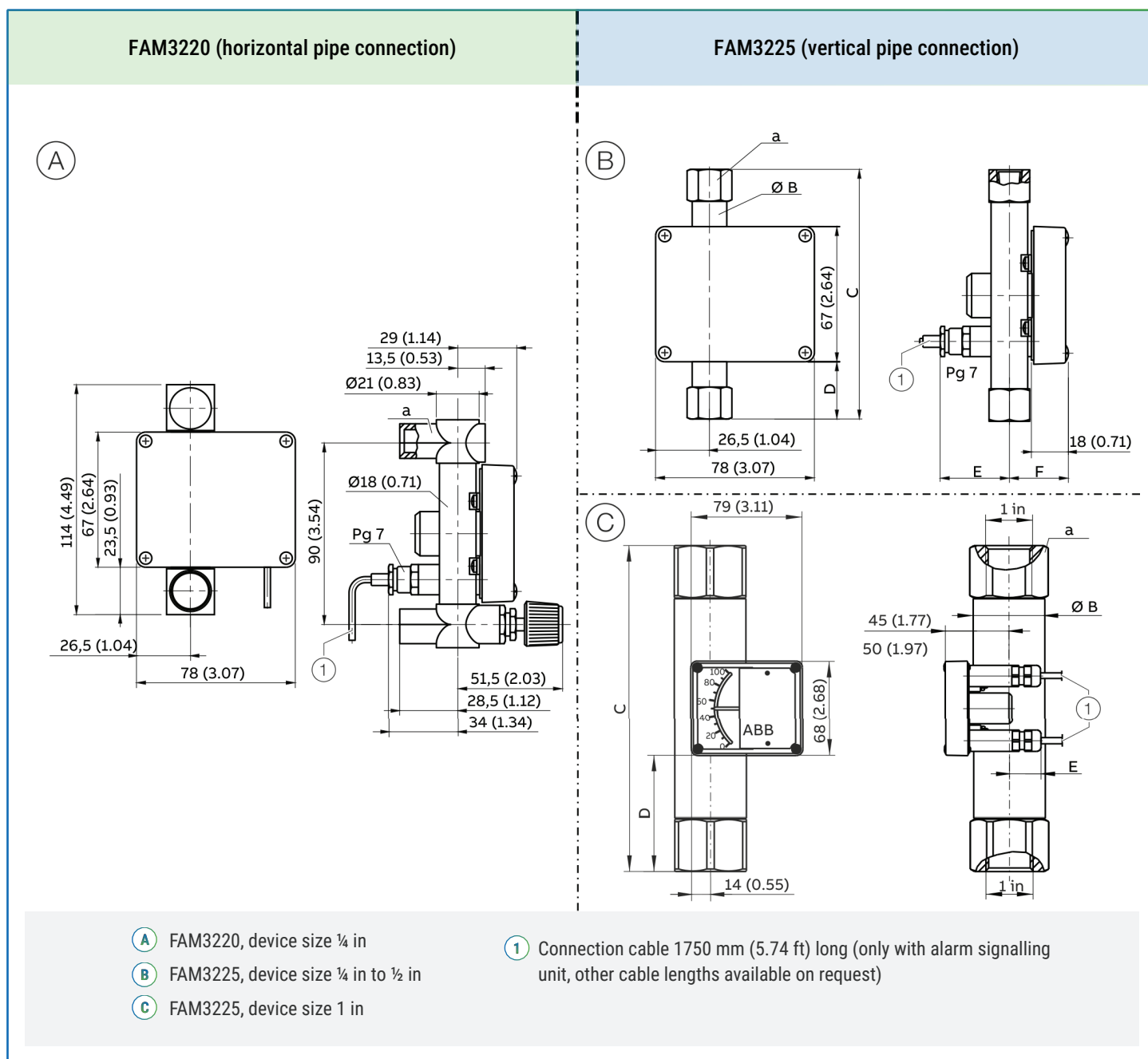
Figure 7: Dimensions in mm (in), projection in accordance with ISO method E, SW width across flats in mm
