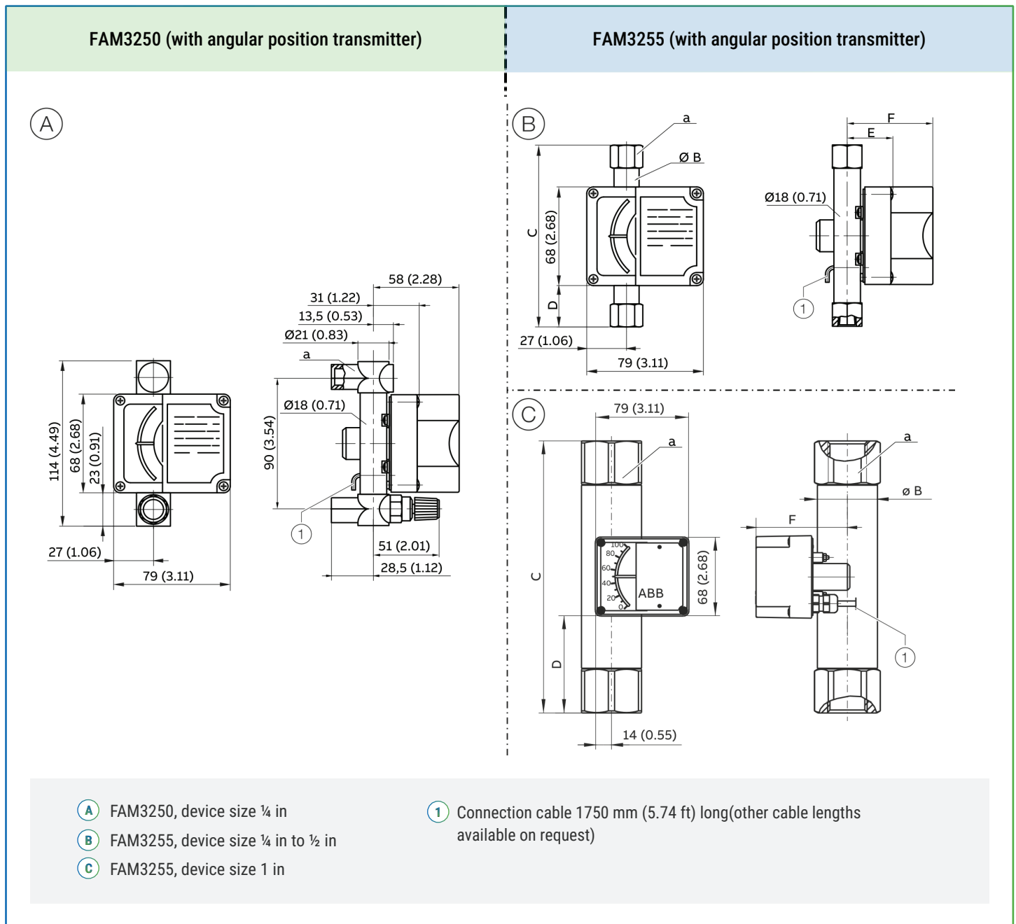
Figure 8: Dimensions in mm (in), projection in accordance with ISO method E, SW width across flats in mm
