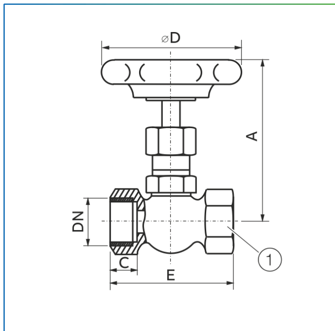
Figure 11: Brass needle valve
